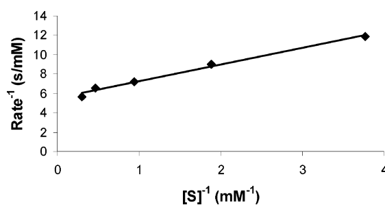
FIGURE 3. Lineweaver-Burk plot of 9a as the substrate of \beta -glucosidase. \beta -Glucosidase (0.5 mg/mL) and substrate ([S]) 9a (0.1, 0.2, 0.4, 0.8, 1.25 mg/mL) were incubated in 150 mM Tris-CF 3 COOH buffer for 10 s at pH 7.30.
