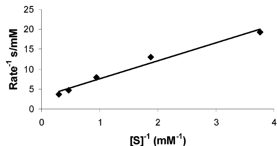
FIGURE 4. Lineweaver–Burk plot of 9b as the substrate of \beta -galactosidase. \beta -Galactosidase (0.5 mg/mL) and substrate ([S]) 9b (0.1, 0.2, 0.4, 0.8, 1.25 mg/mL) were incubated in 150 mM Tris- \text{CF}_3\text{COOH} buffer for 10 s at pH 7.30.
